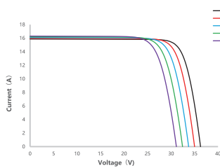
I-V Curve at Different Temperature SSA-48HDB-445N
